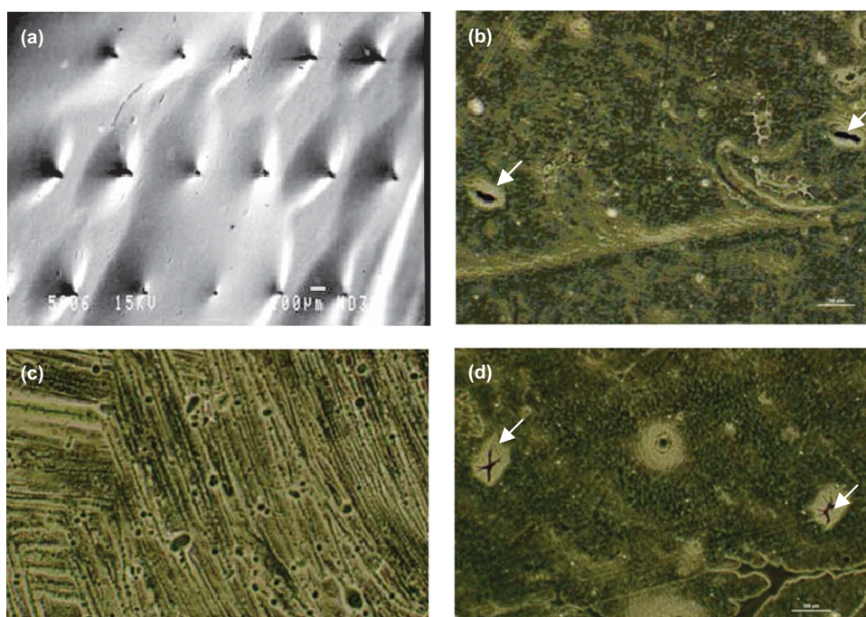
Figure 6. Image showing galactose MN puncturing the Silescol ® membrane (a). Holes created in Silescol ® membrane upon immediate removal of galactose MNs (b). Silescol ® membrane following the 6-hour application of galactose MNs (c). Silescol ® membrane 6 hours after the removal of galactose MNs. Image a was taken using a JEOL JSM840 scanning electron microscope (Jeol) and images b, c, and d were obtained using an ECLIPSE TE300 inverted microscope with a DXM1200 digital still camera (Nikon, UK Ltd., Kingston upon Thames Surrey, UK).
