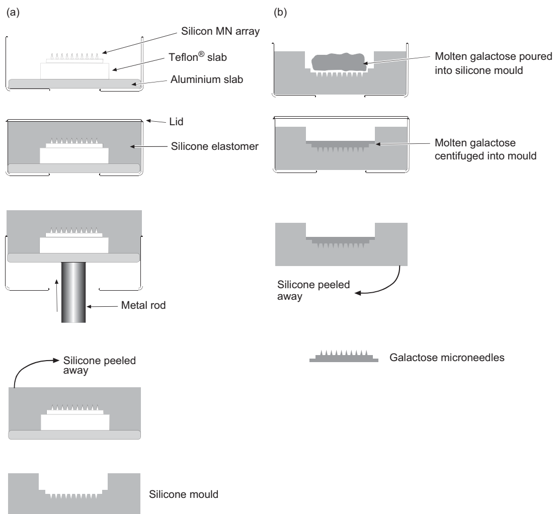
Figure 2. Diagrammatic representation of the steps involved in the preparation of galactose microneedles, showing first production of silicone master moulds from silicon microneedle arrays (a) and second preparation of galactose microneedle arrays from silicone master moulds (b).
